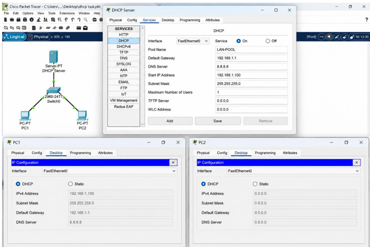
Figure : DHCP Server and Client IP Configuration.
